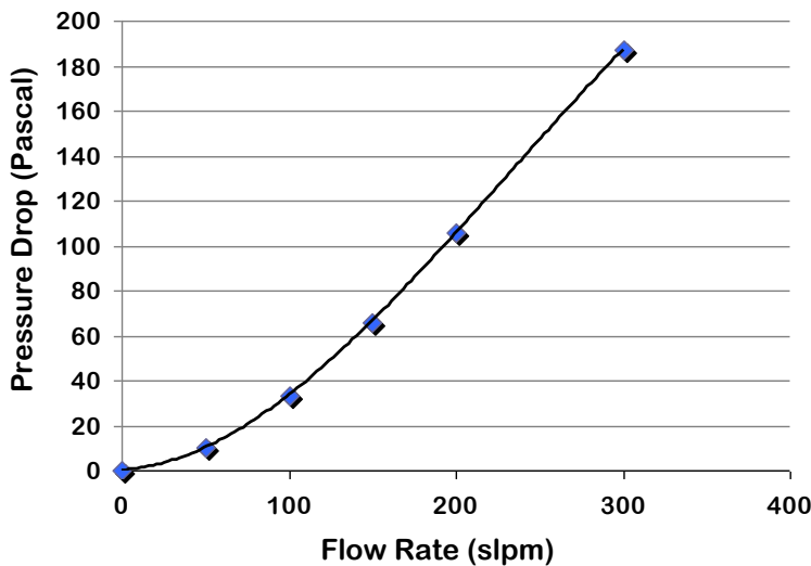
PMF4104V Pressure Drop
